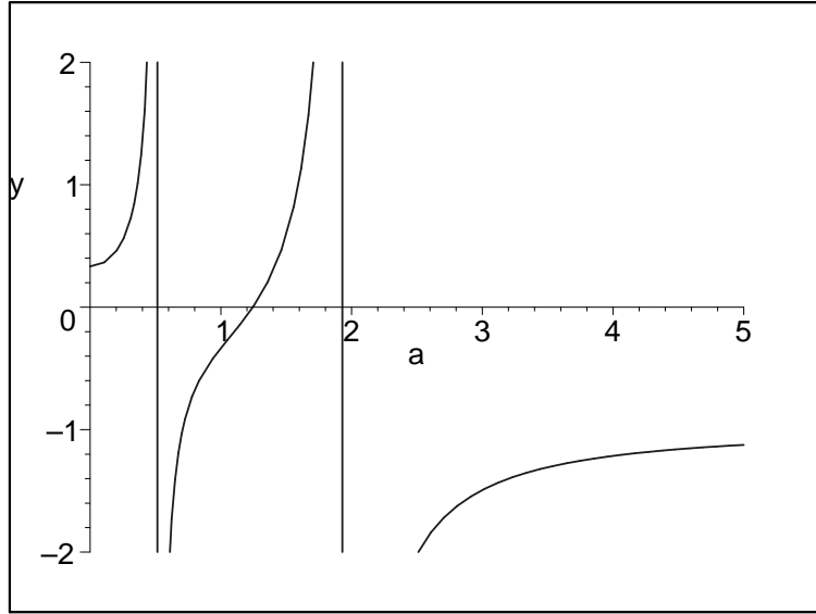
Figure 4. Plot of equation of state parameter w_{D.E.} vs. scale factor a(t) for \omega^2 > \Lambda_W^2 , k\omega < 0 . There are two infinite discontinuities of w_{D.E.} at \tilde{a}^\pm = \sqrt{-k\omega \pm |k|\sqrt{\omega^2 - \Lambda_W^2}}/|\Lambda_W|R_0 where \rho_{D.E.} vanishes. Here, I considered |\omega|R_0^2 = 2 , |\Lambda_W|R_0^2 = 1 case ( \omega R_0^2 = -2, k = +1 or \omega R_0^2 = +2, k = -1 ).
