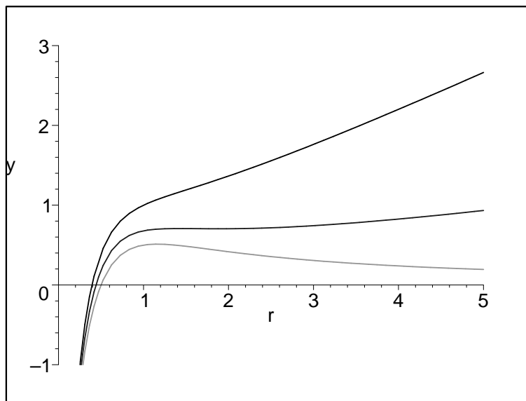
Figure 1. Plots of 4\pi T vs. black hole’s outer horizon radius r_+ for various \Lambda_W , i.e., \Lambda_W = -1, 0.5, 0 (top to bottom) with \omega = 2 . For large black holes, the temperature interpolates between the AdS cases (above two curves) and flat (bottom curve). In IR region, i.e., small black holes, there exists an extremal black hole limit of the vanishing temperature at r_+^* in which r_- meets with the outer horizon r_+ . The region smaller than the extremal radius, which being the Cauchy horizon, shows an unphysical negative temperature.
