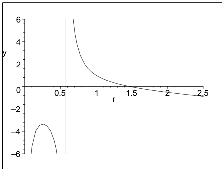
Figure 2. Plots of 4\pi T vs. black hole horizon radius r_+ for the dS black hole case with \Lambda_W = +1 and \omega = -2 . There exists also an extremal limit of the vanishing temperature at r_+^* of (17) in which the black hole horizon r_+ coincides with the cosmological horizon r_{++} , i.e., the Nariai limit. There is an infinite discontinuity of temperature at \tilde{r}_+ = 1/\sqrt{\Lambda_W - \omega} .
