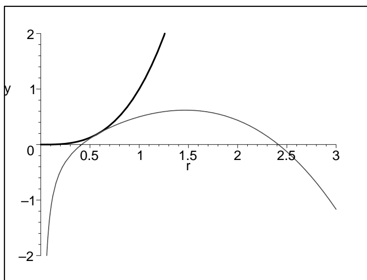
Figure 3. Plots of mass spectrum M of (24) (lower curve) vs. the upper mass bound M = \frac{(2\Lambda_W - \omega)}{4} r_+^3 of (23) (upper curve) for the existence of black hole horizon r_+ . This shows that the mass bound is always satisfied for all horizon radius r_+ and this is saturated at the point r_+ = 1/\sqrt{\Lambda_W - \omega} = \tilde{r}_+ . And also, the mass parameter gets the maximum value in the spectrum at the Nariai limit r_+^* . Here I plotted \Lambda_W = +1 and \omega = -2 cases but the results are generally valid for arbitrary values of \Lambda_W > 0 and \omega < 0 .
