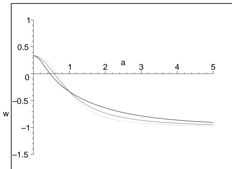
Figure 7. Plots of equation of state parameters w_{D.E.} vs. scale factor a(t) for k\omega > 0 ( \omega R_0^2 = +2, +1, +1/2 , k = +1 or \omega R_0^2 = -2, -1, -1/2 , k = -1 with |\Lambda_W|R_0^2 = 1 (top to bottom in the left region)). In this case, w_{D.E.} is “always” monotonically decreasing from 1/3 in the UV limit to -1 in the IR limit.
