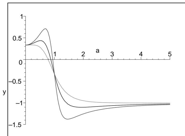
Figure 6. Plots of equation of state parameters w_{D.E.} vs. scale factor a(t) for \omega^2 < \Lambda_W^2 , k\omega < 0 ( \omega R_0^2 = +1/1.3, +1/2, +1/10 , k = -1 or \omega R_0^2 = -1/1.3, -1/2, -1/10 , k = +1 with |\Lambda_W|R_0^2 = 1 (top to bottom in the left region)). When |\omega| is not far from |\Lambda_W| , there is a region where w_{D.E.} is fluctuating beyond the UV and IR limits and this can be understood as a smooth deformation of the plot of figure 5. When |\omega| is small enough, w_{D.E.} is monotonically decreasing from 1/3 in the UV limit to -1 in the IR limit.
