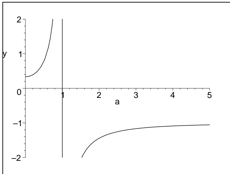
Figure 5. Plot of equation of state parameter w_{D.E.} vs. scale factor a(t) for \omega^2 = \Lambda_W^2 , k\omega < 0 . The two points of infinite discontinuities \tilde{a}^\pm in figure 4 merge as |\omega| approaches to |\Lambda_W| and they meet at \tilde{a}^\pm = \sqrt{|k|}/|\Lambda_W|R_0 when \omega^2 = \Lambda_W^2 . In this plot, I considered |\omega|R_0^2 = |\Lambda_W|R_0^2 = 1 ( \omega R_0^2 = -1, k = +1 or \omega R_0^2 = +1, k = -1 ).
